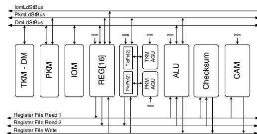
Figure 2. Initial ASIP Data Path
