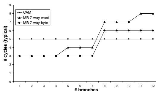
Figure 4. Multibranch solutions compared
