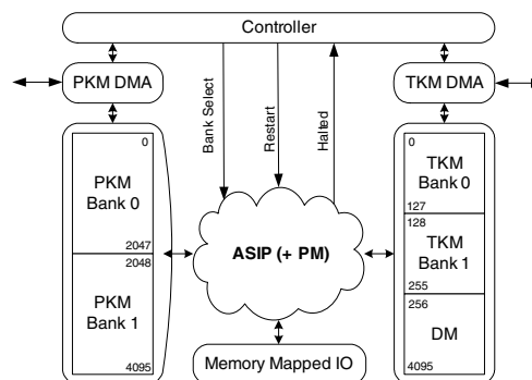
Figure 1. External ASIP interfaces
