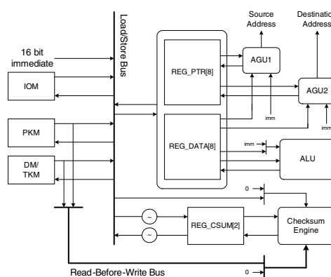
Figure 3. ASIP Data path final design
